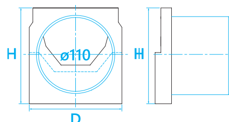
Endcap with pipe
